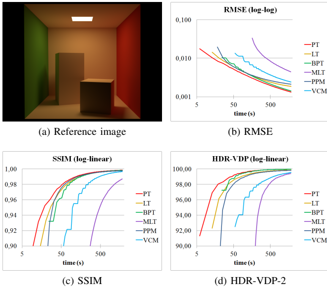
Fig. 2. Reference image and results for test scene Cornell Box Diffuse.
